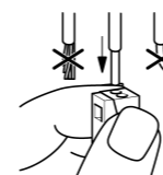
Figure 8: Connection of the single-stranded cable
